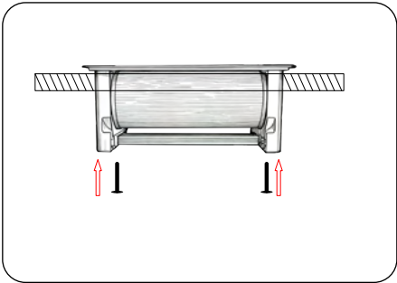
2. Insert Screws Insert long screws diagonally from the bottom.
