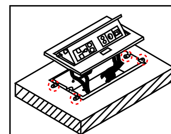
3.Fix Housing Insert the housing into the desk cutout and secure with 4 self-tapping screws. (Tip: Keep power and data cables separated.)
