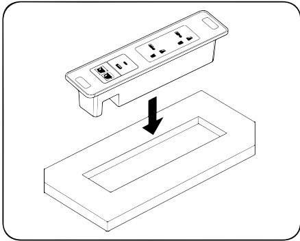
248×55 mm Desk Cut-out & Insert Unit
